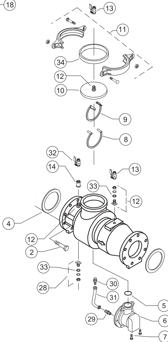
MODEL 375 (65mm - 80mm)
