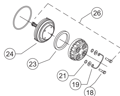
#1 CHECK ASSEMBLY (375 100mm - 150mm) (375A 100mm - 150mm)
