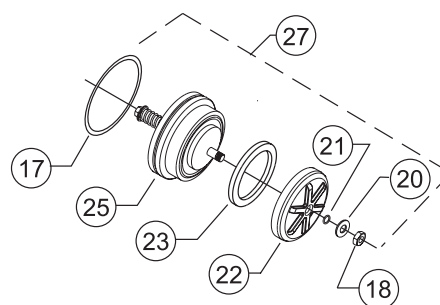
#2 CHECK ASSEMBLY (375 & 475 65mm - 80mm)
