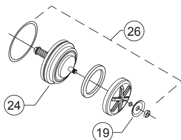
#1 CHECK ASSEMBLY (350 & 450 65mm - 80mm)
