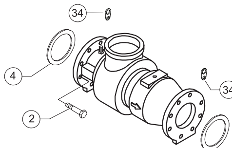
MODEL 375 (100mm - 250mm)
