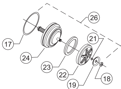
#1 CHECK ASSEMBLY (375 & 475 65mm - 80mm)
