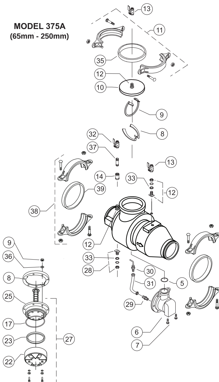
#2 CHECK ASSEMBLY (375 & 375A 200mm - 250mm)
