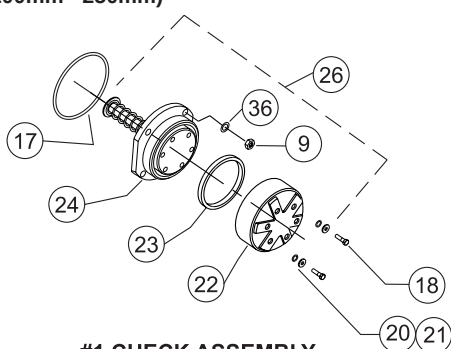
#1 CHECK ASSEMBLY (375 & 375A 200mm - 250mm)
