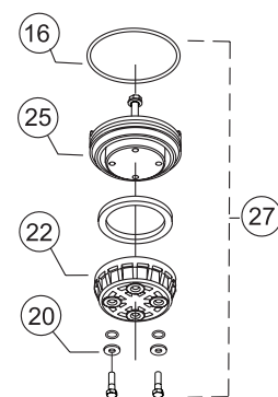
#2 CHECK ASSEMBLY (350 100mm - 250mm) (350A 65mm - 300mm)
