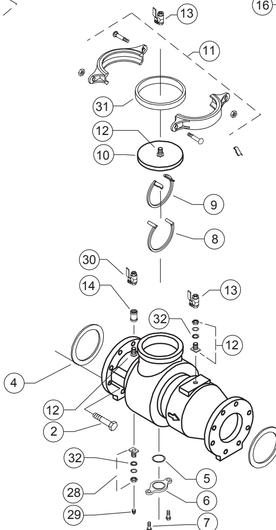
MODEL 350 (65mm - 80mm)
