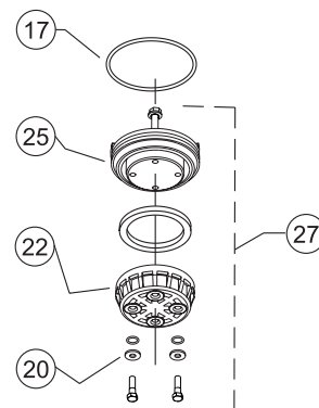
#2 CHECK ASSEMBLY (375 100mm - 150mm) (375A 100mm - 150mm)
