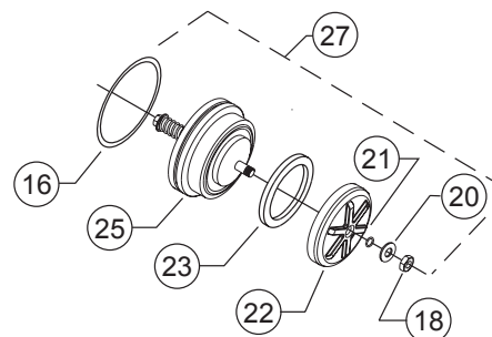
#2 CHECK ASSEMBLY (350 & 450 65mm - 80mm)
