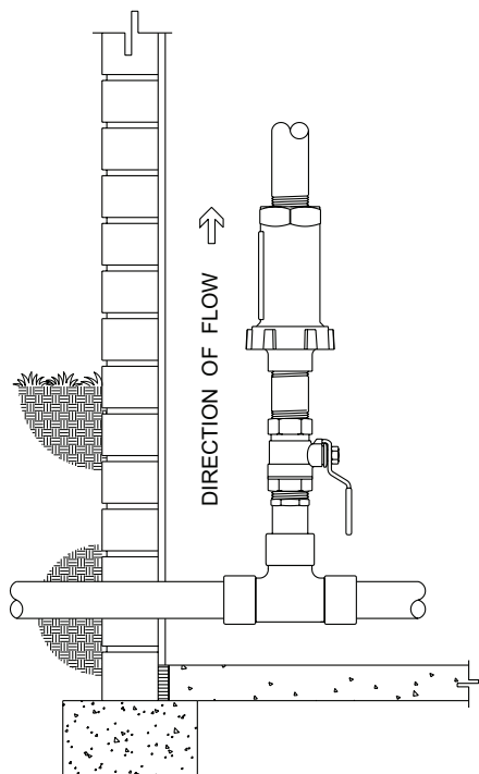
VERTICAL INSTALLATION
