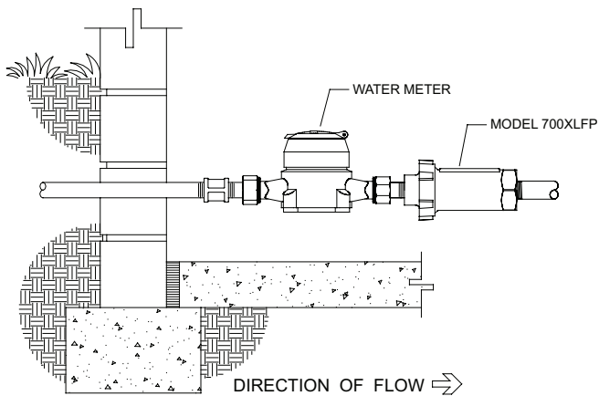
INDOOR INSTALLATION
