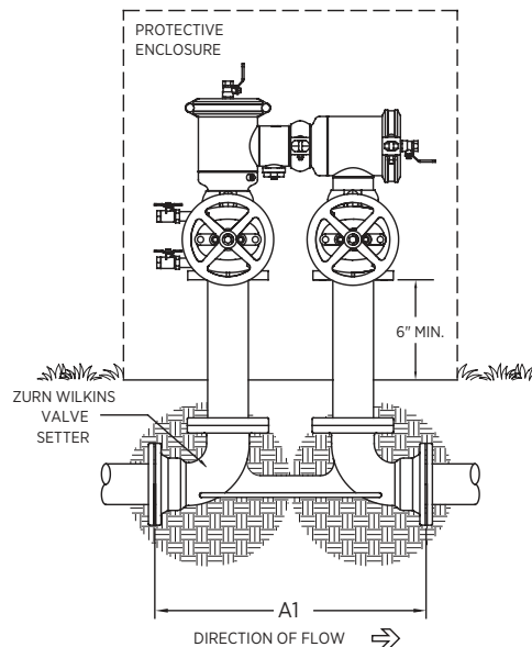
OUTDOOR INSTALLATION
