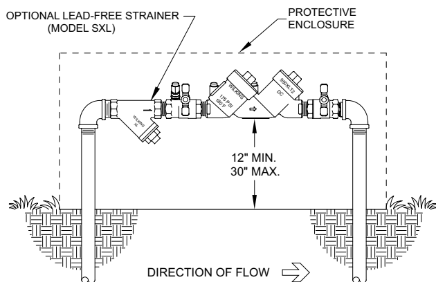
MODEL 950XLT2S
