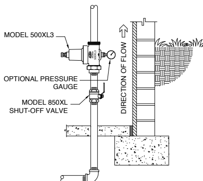
VERTICAL INSTALLATION
