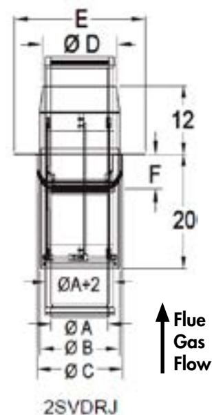
DOUBLE WALL
