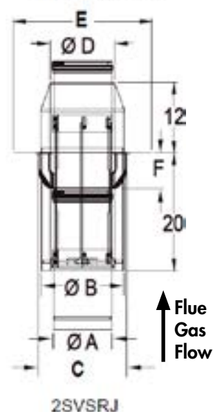
SINGLE WALL
