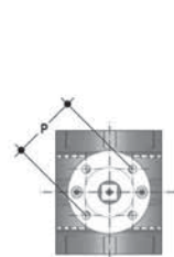
Dimensions (inches)
