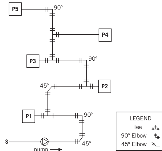
Figure 1 – Schematic of Simple System Loop
