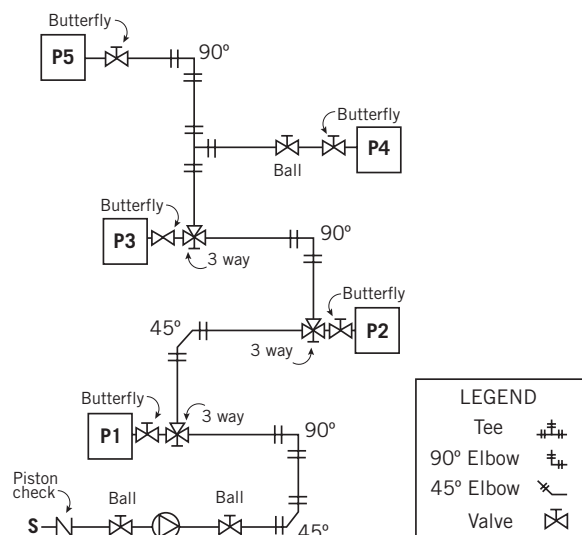
Figure 2 - Schematic of Simple System Loop with Valves
