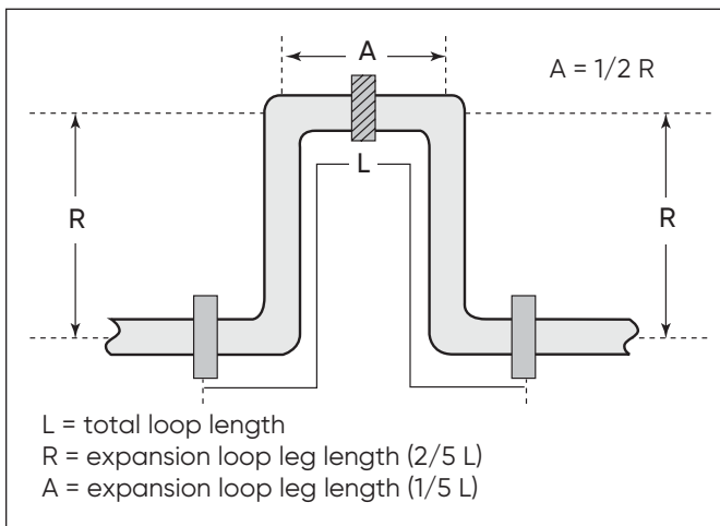
Expansion Loop
