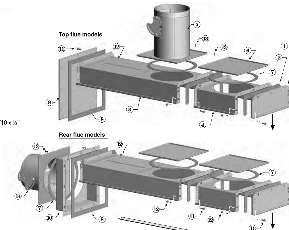
Figure 10 Flue collector components, typical (Model 880 collector configurations shown)
