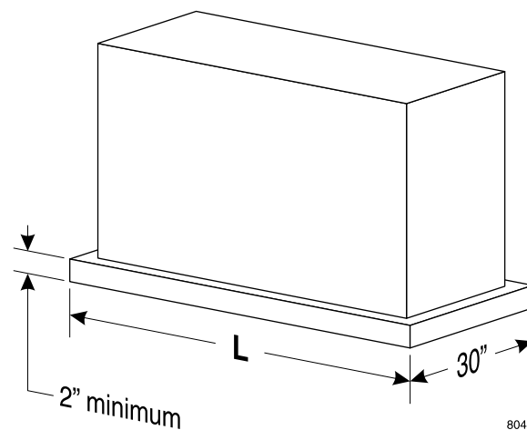
Figure 1 Boiler foundation
