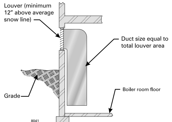
Figure 3 Combustion and ventilation air openings — Boiler room partially or completely above grade
