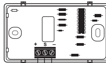
Remote Sensor
