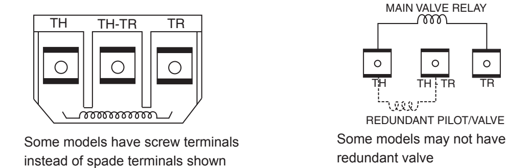
Milivolt 3 Terminal Panel Fig. 2
