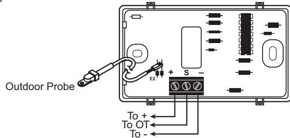
Remote Outdoor Sensor Base
