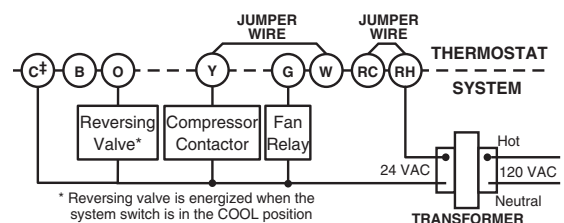
Heat pump with reversing valve energized in COOL
