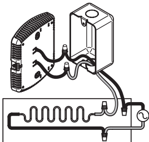
4 Wire Installation
