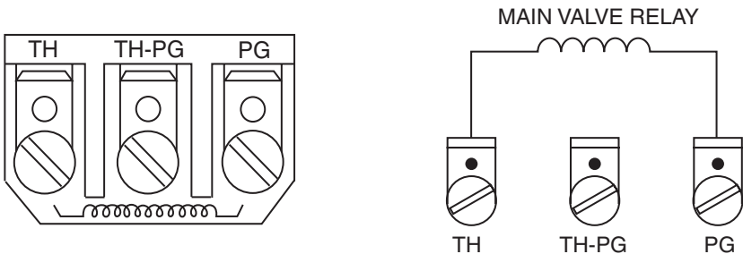
Milivolt 3 Terminal Panel Fig. 2
