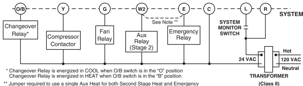
Single transformer systems
