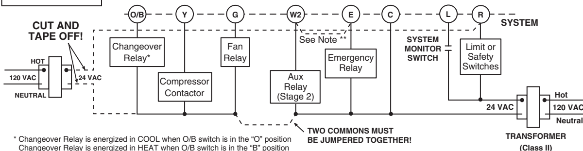
Two transformer systems with NO safety circuits
