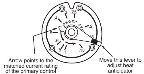
Anticipator adjustment
