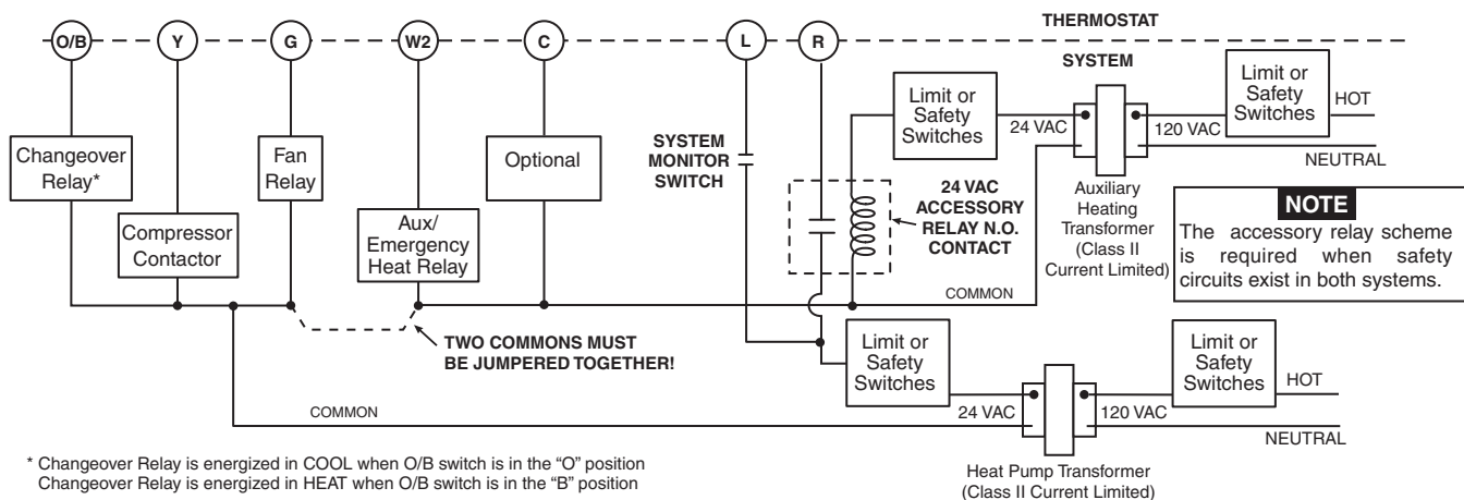
Typical wiring diagram for two transformer systems with safety circuits in BOTH systems
