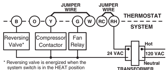
Heat pump with heat active reversing valve
