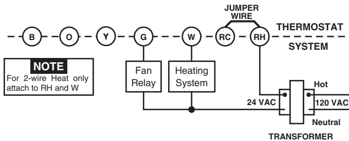
Heat only, 3-wire, single transformer systems
