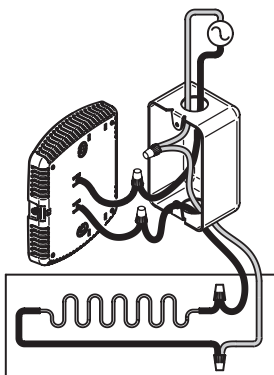
4 Wire Installation
