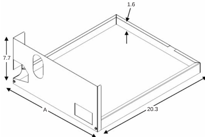
FIGURE 19 UNCASED COIL ADAPTER KIT ILLUSTRATION
