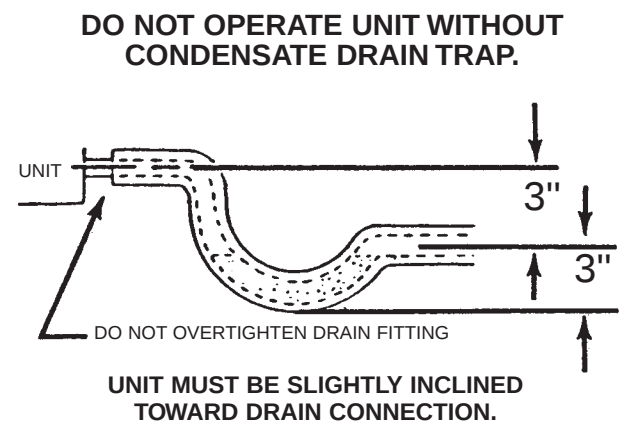
FIGURE 15 CONDENSATE DRAIN TRAP
