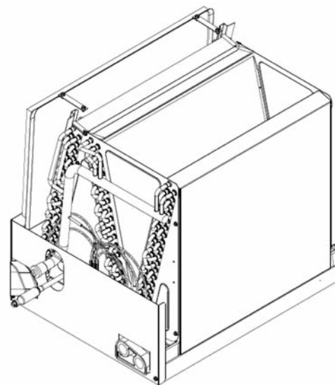
FIGURE 20 UNCASED COIL ADAPTER KIT ASSEMBLED
