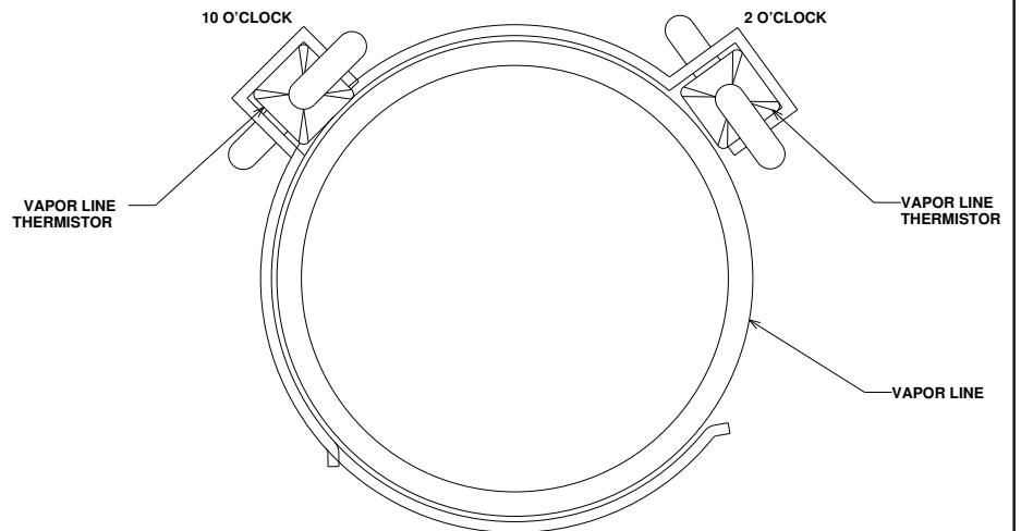
FIGURE 9 THERMISTER LOCATION
