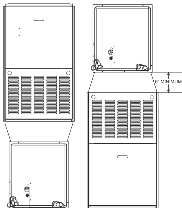
FIGURE 5B INSTALLATION OF COIL MATCH WITH A FURNACE ONE SIZE SMALLER
