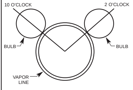
FIGURE 8 BULB LOCATION
