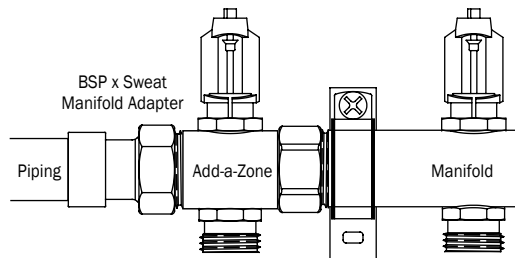
An Add-a-Zone attached to the end of a Stainless Steel supply manifold to increase capacity.
