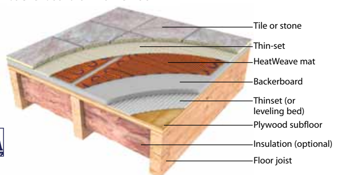
HeatWeave mat in thin-set on backboard on frame floor
