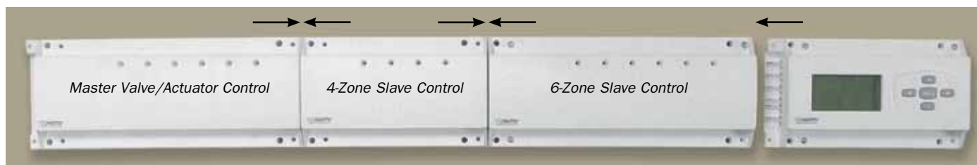
Master Valve/Actuator Control unit mated to 4-Zone and 6-Zone Slave Control units with an optional Timer.
