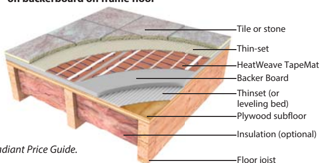
HeatWeave TapeMat in thin-set on backerboard on frame floor
