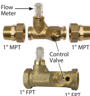
1" FPT
