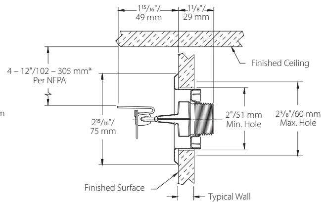
MAXIMUM RECESS
