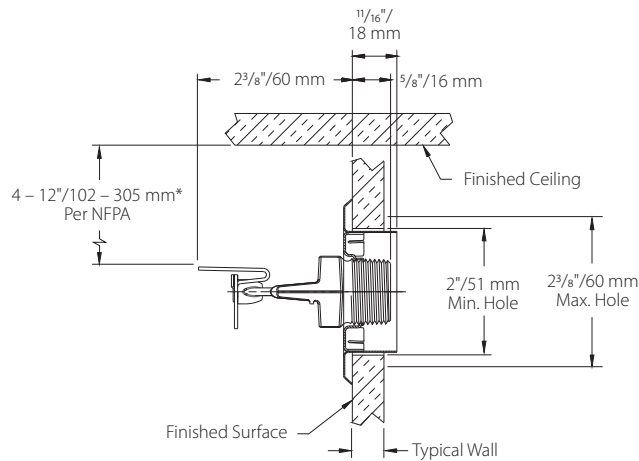
MAXIMUM EXTENSION
