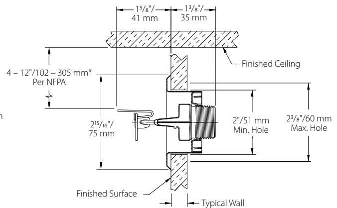
MAXIMUM RECESS
