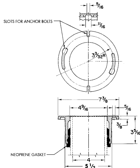
2-252TY* Push-On Closet Flange
