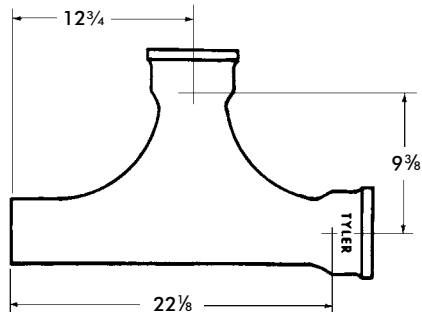
TWO-WAY CLEANOUT Memphis Code
