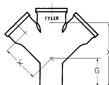
DOUBLE WYE
