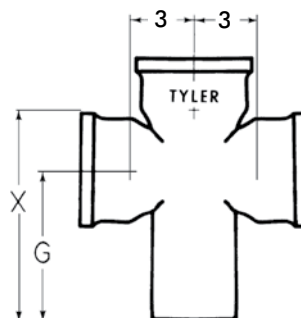
STRAIGHT CROSS
