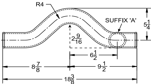
By-Pass Fitting
