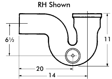
"P" TRAP W/¾" CLEANOUT TAP, R, L
