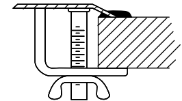
Stud Mounting Provides Easy Installation
