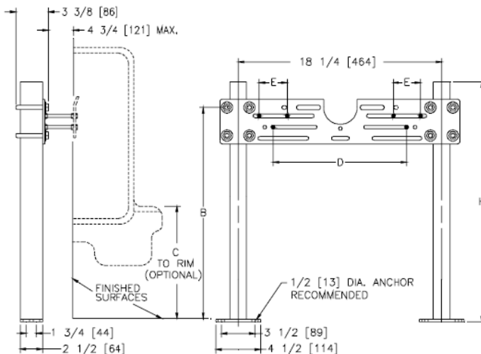
HW5020 Hardware Bearing Plate part #S4101
