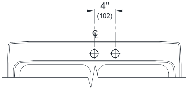
-2R Single Hole Centered with 2nd Hole 4" to Right
