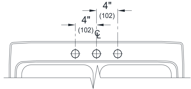
-3 Three Holes on 4" Centers (8" Centerset)
