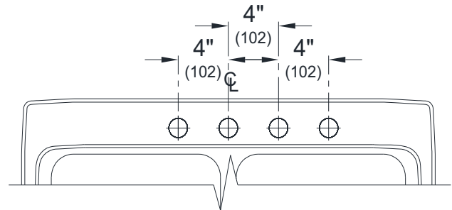
-4R Three Holes on 4" Centers with 4th Hole 4" to Right
