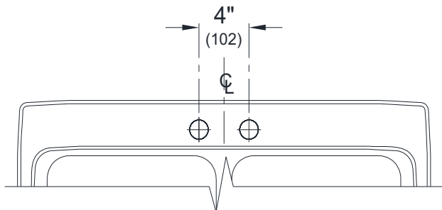
-2 Two Holes on 4" Centers (4" Centerset)
