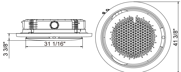
Open Type
