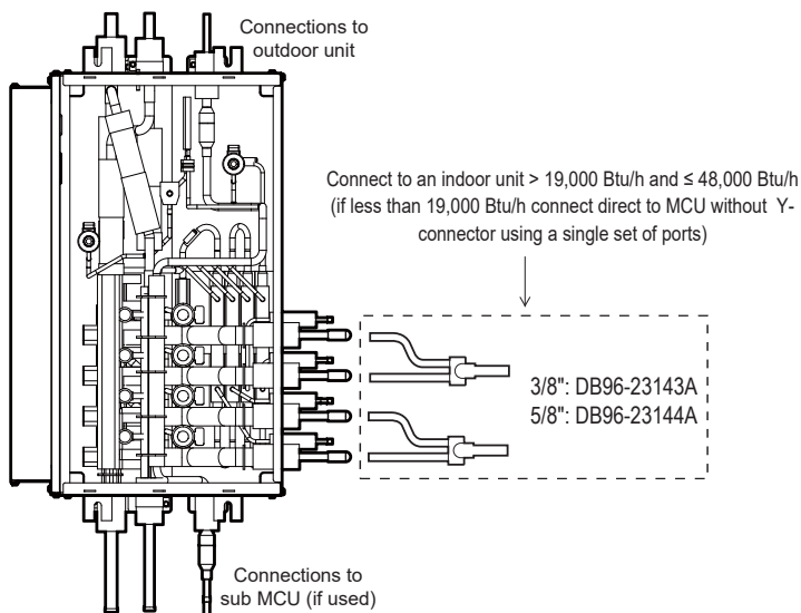
TOP VIEW (PICTURED WITHOUT COVER)
