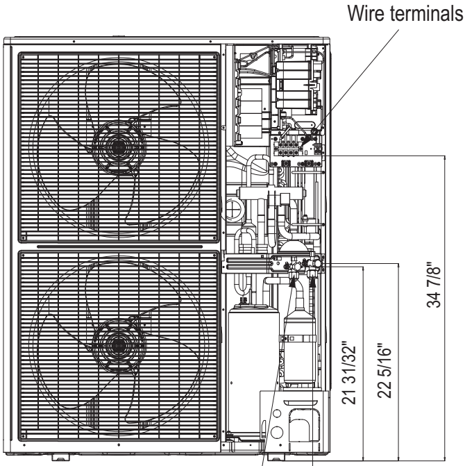
FRONT (W/O PANEL)
