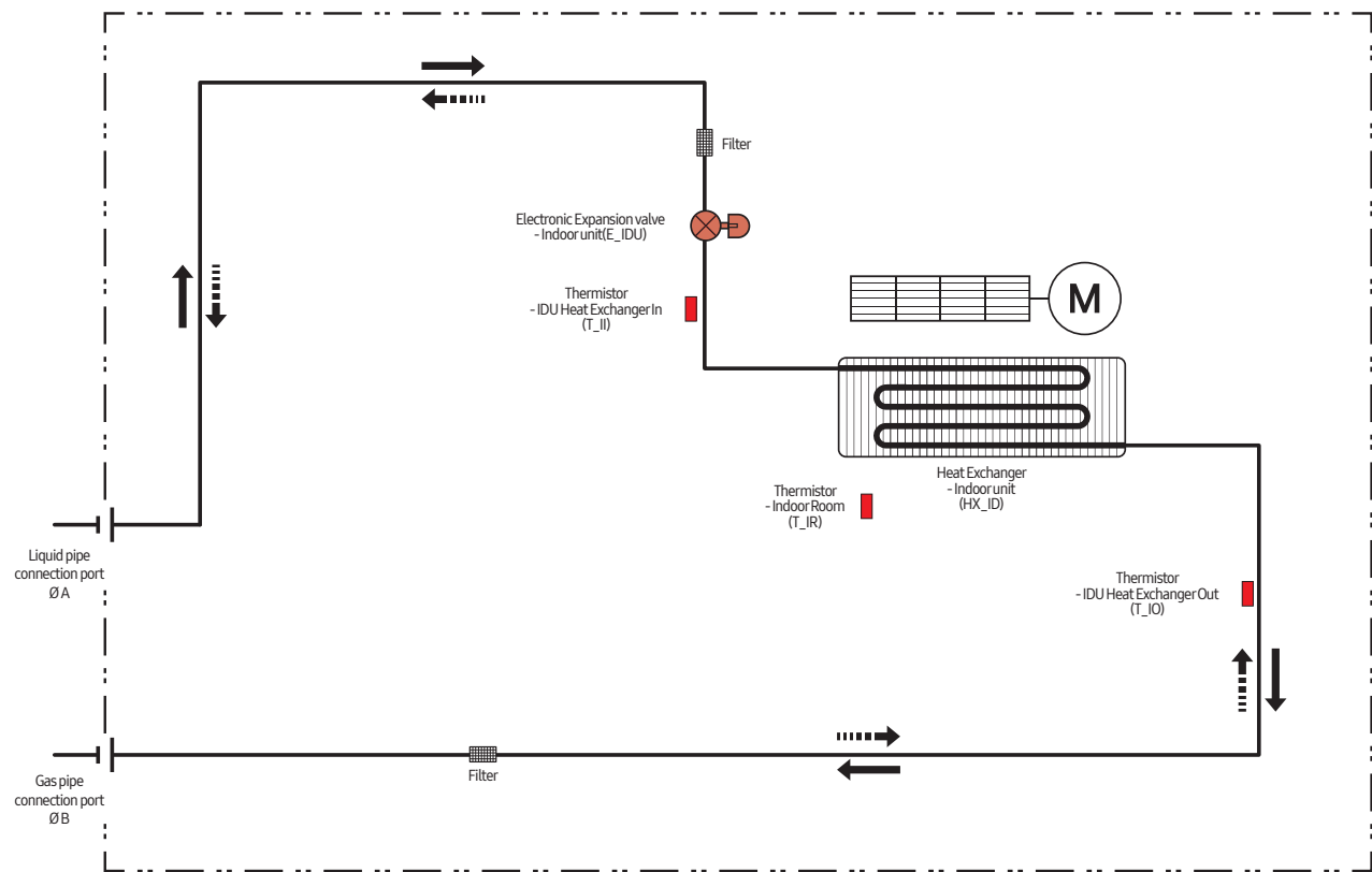
EEV included Model
