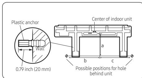
Pipe bundle hole: 2.56 inch (Ø65 mm) (Unit: inch (mm))
