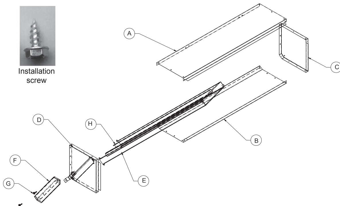
Assembly screw
