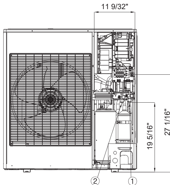
FRONT WITHOUT SERVICE COVER
