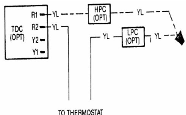
FIGURE 2 WIRING
