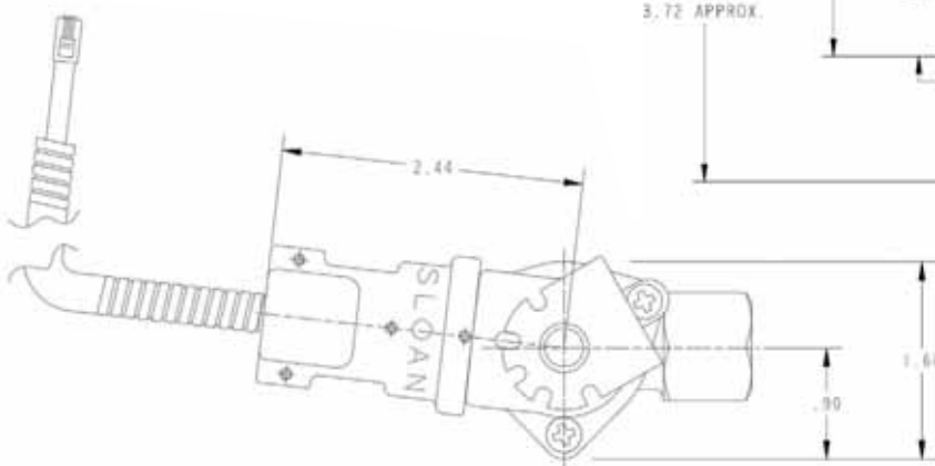
S-45 with Connector
