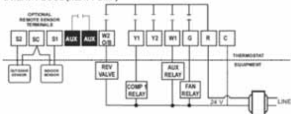
2 HEAT/1 COOL (HEAT PUMP)
