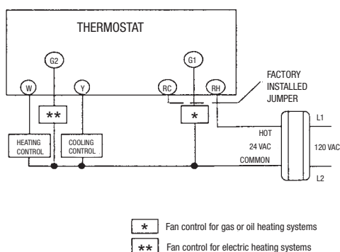
One Transformer - Models PS986-1R, PS988-1R
