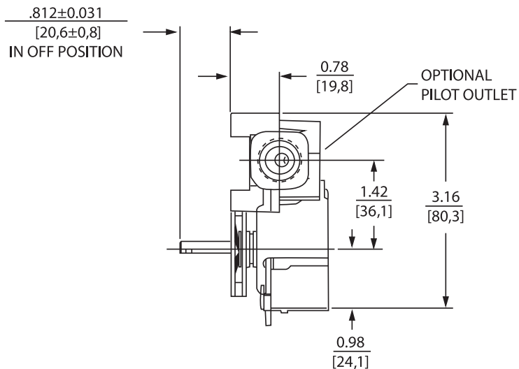
Right View
