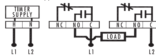
208/240VAC Application
