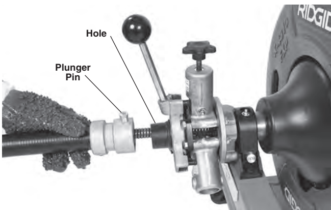
Figure 10 – Attaching Front Guide Hose
