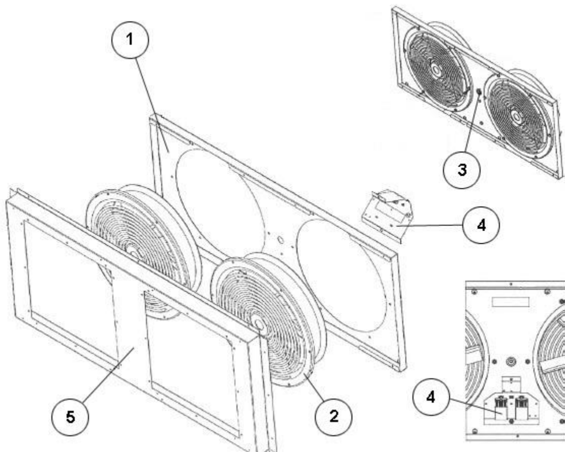
CDF01D Assembly
