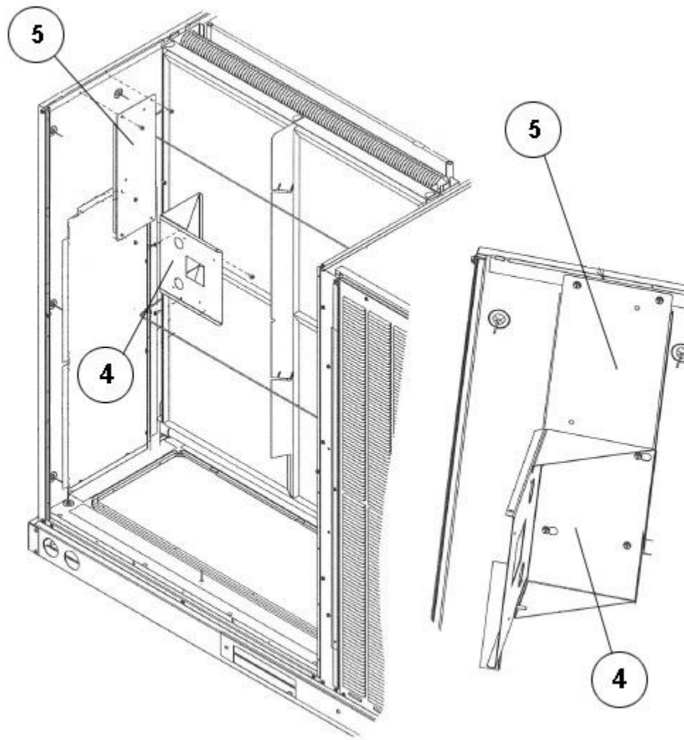
RXRX-BS04 (3) Assembly
