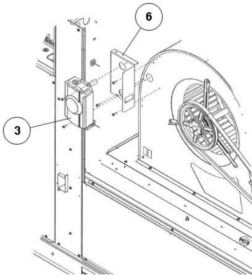
RXRX-BS04 (2) Assembly
