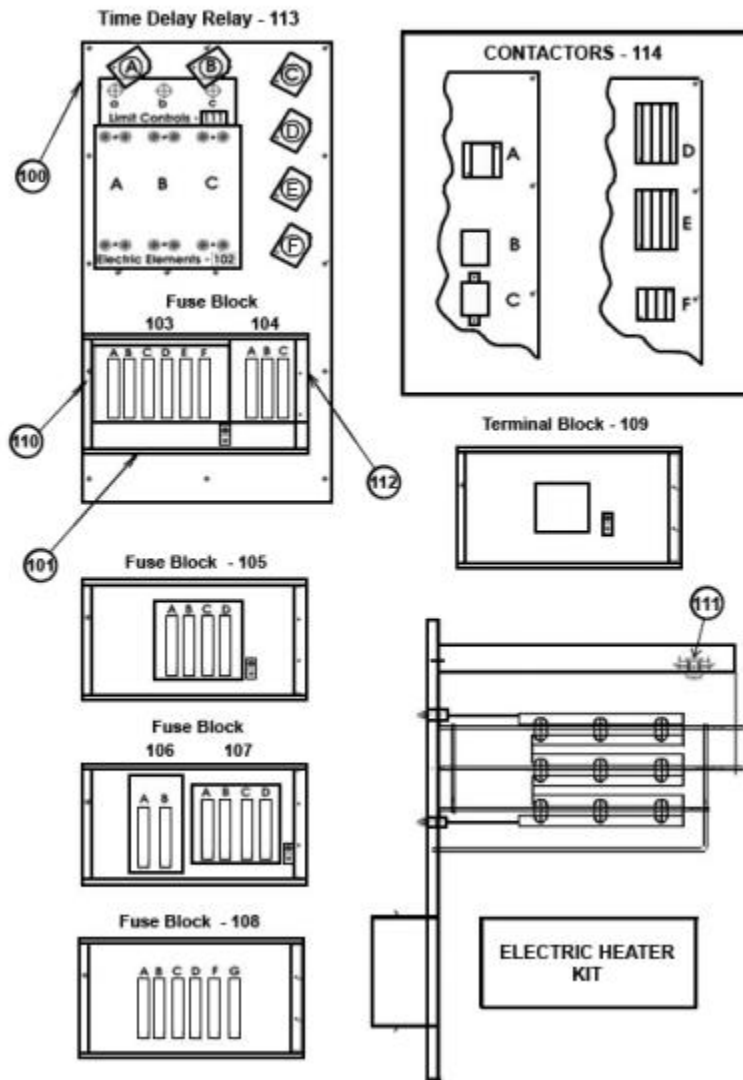
RXJJ-Axxx Assembly
