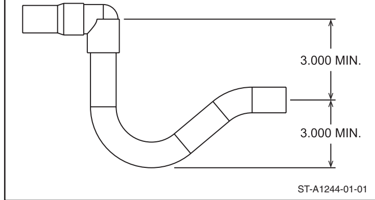
FIGURE 6 CONDENSATE DRAIN TRAP
