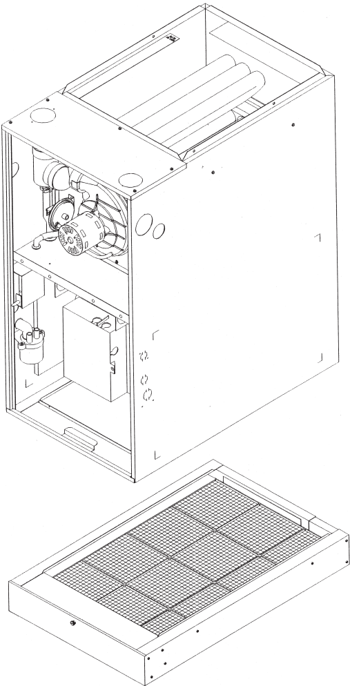
FIGURE 3. UPFLOW BOTTOM MOUNT – RXGF-CB
