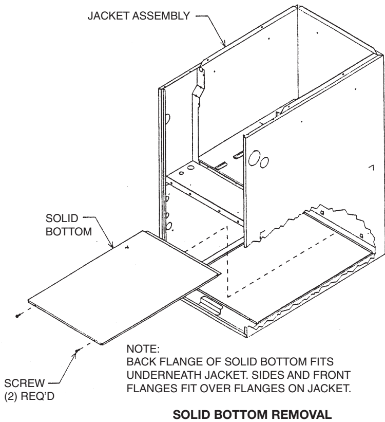
FIGURE 2. BOTTOM PANEL REMOVAL
