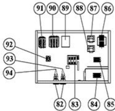
Control Panel 200
