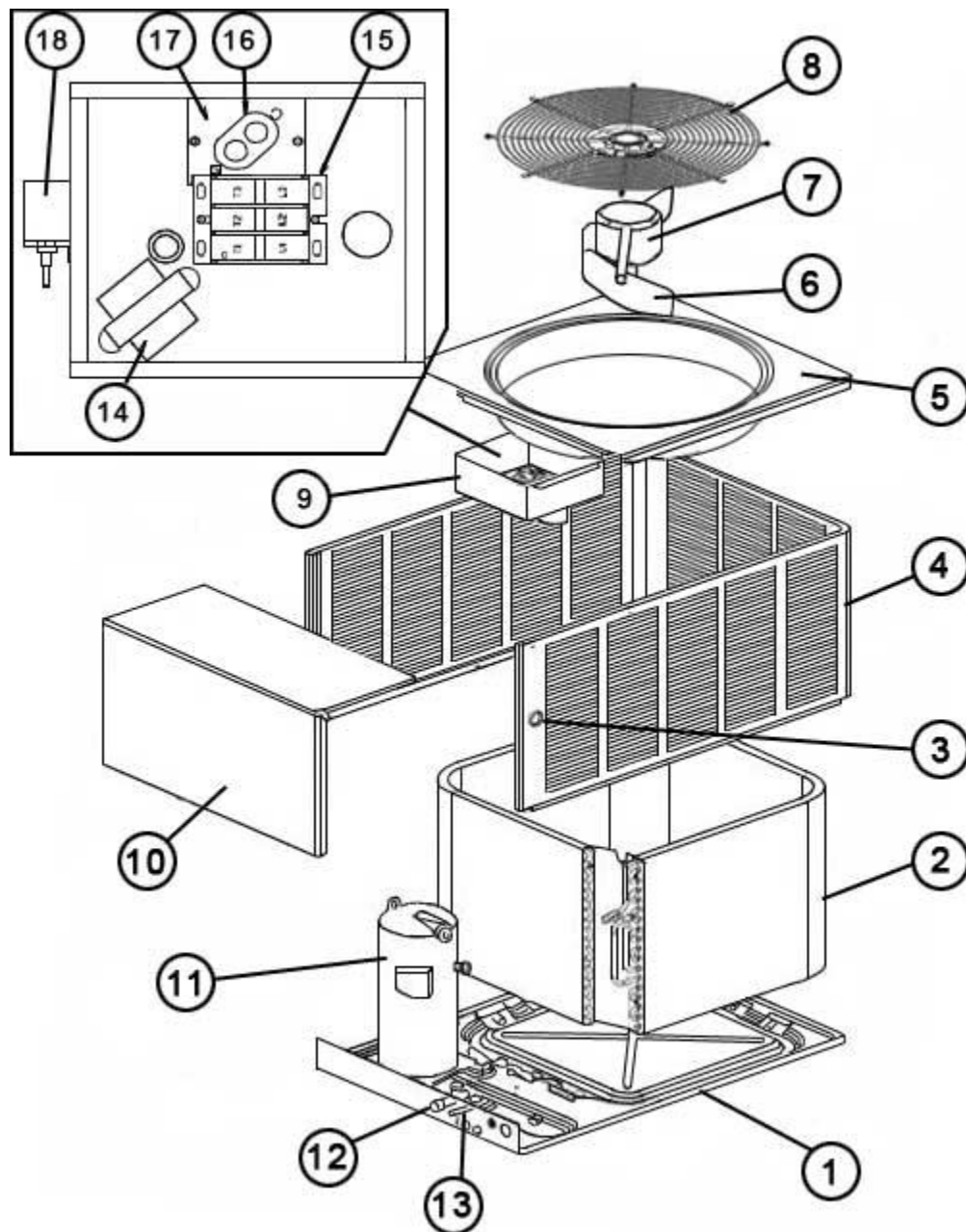
Exploded View 078-091
