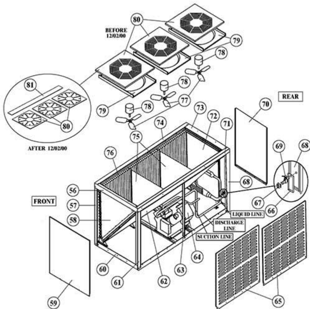
Exploded View 200
