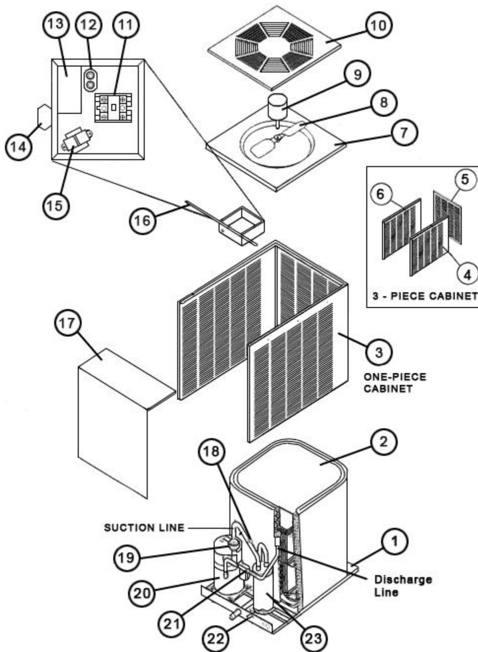
Exploded View 065-076
