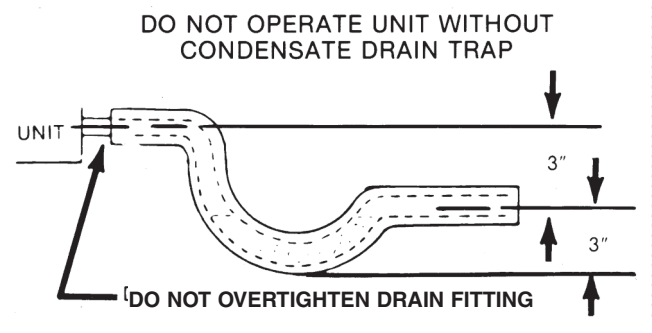
FIGURE 19 CONDENSATE DRAIN
