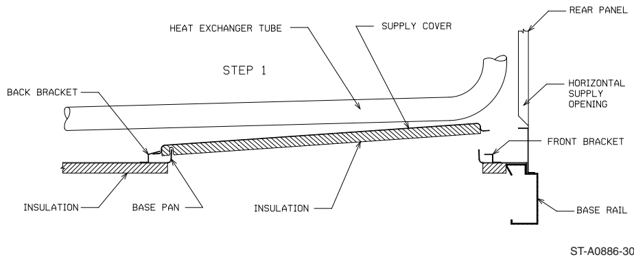
FIGURE 10 HORIZONTAL CONVERSION DETAIL
