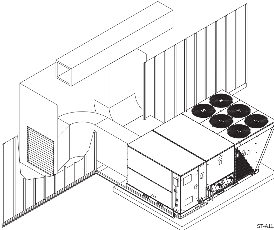
FIGURE 9 OUTSIDE SLAB INSTALLATION. CLOSET DISTRIBUTION SYSTEM. SLAB FLOOR CONSTRUCTION
