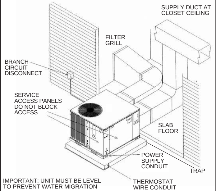
FIGURE 5 PACKAGE AIR CONDITIONER – OUTSIDE SLAB INSTALLATION, CLOSET DISTRIBUTION SYSTEM. SLAB FLOOR CONSTRUCTION.
