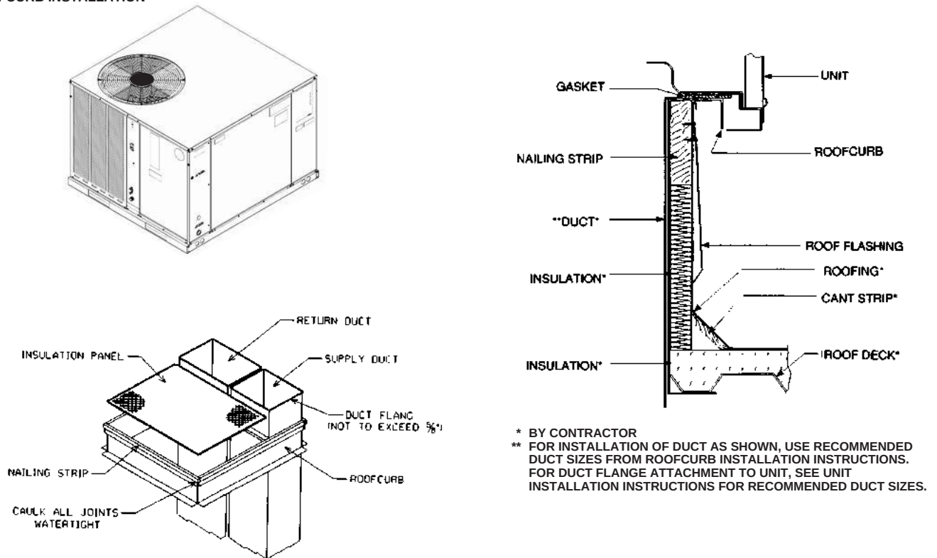
FIGURE 7 ROOFCURB INSTALLATION
