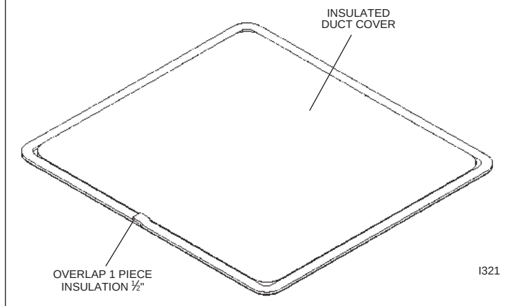
FIGURE 10 COVER GASKET DETAIL
