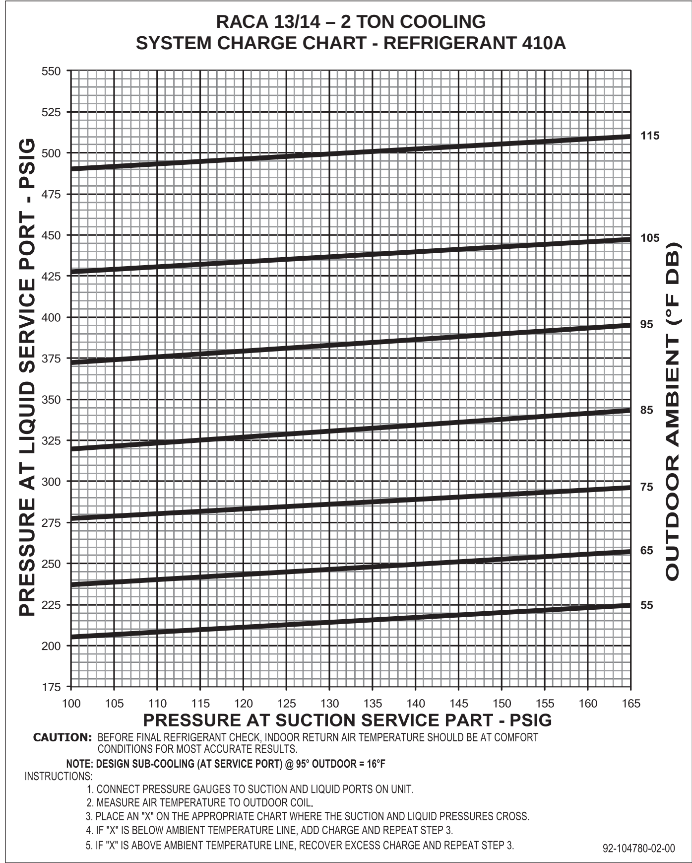
FIGURE 19 SYSTEM CHARGE CHARTS
