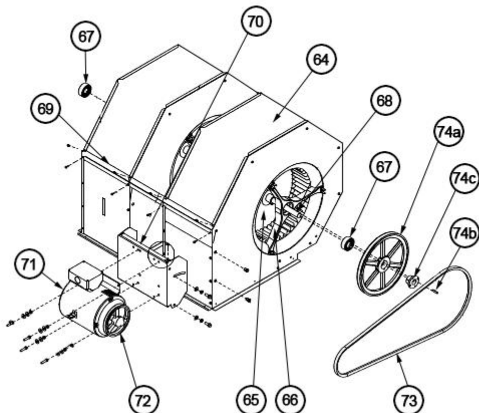
Blower Assembly 180-300
