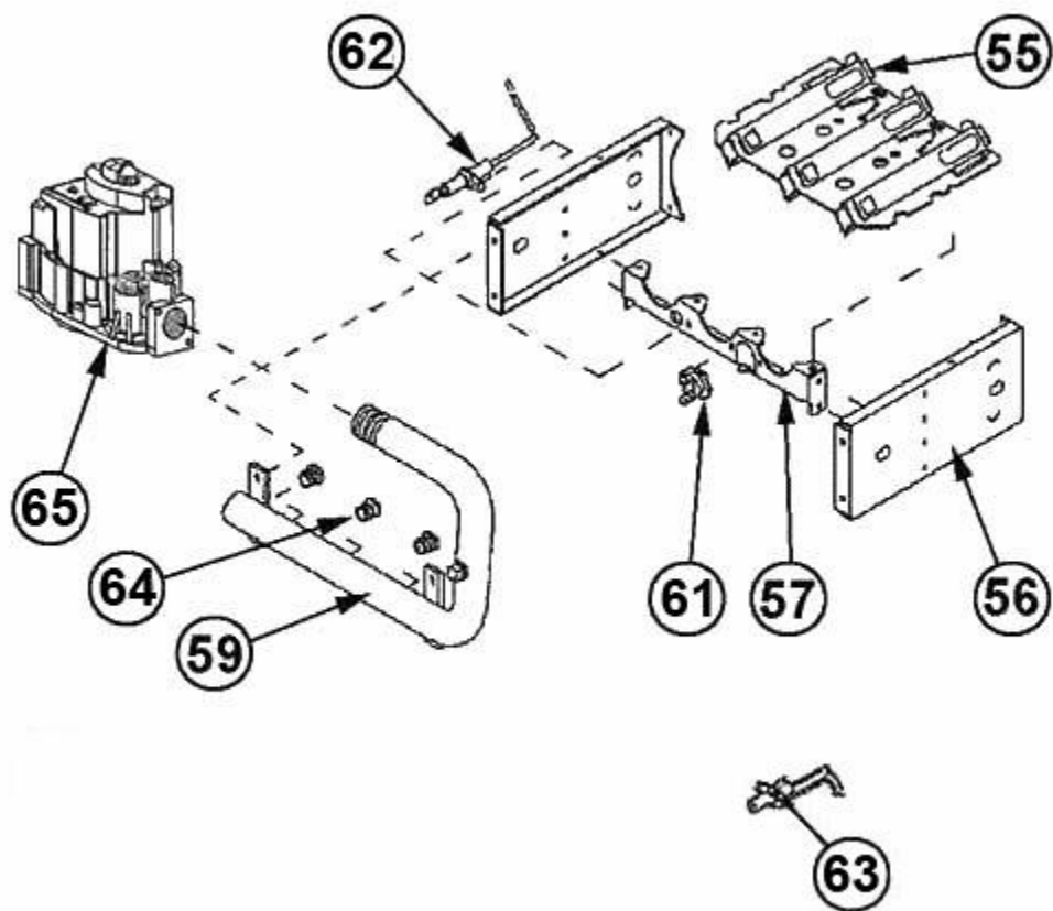
Burner Assembly
