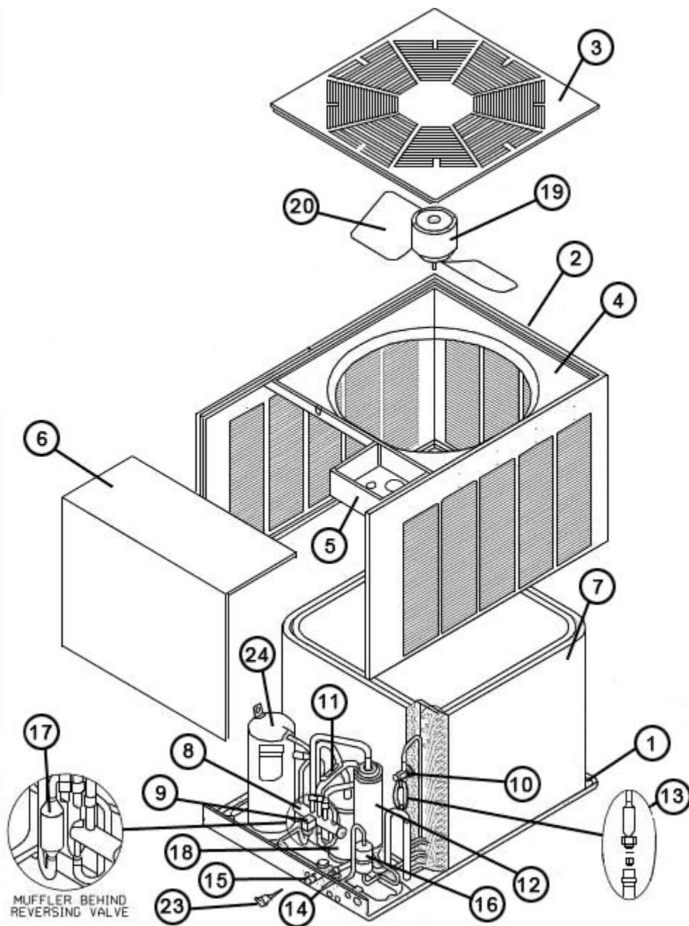
Exploded View
