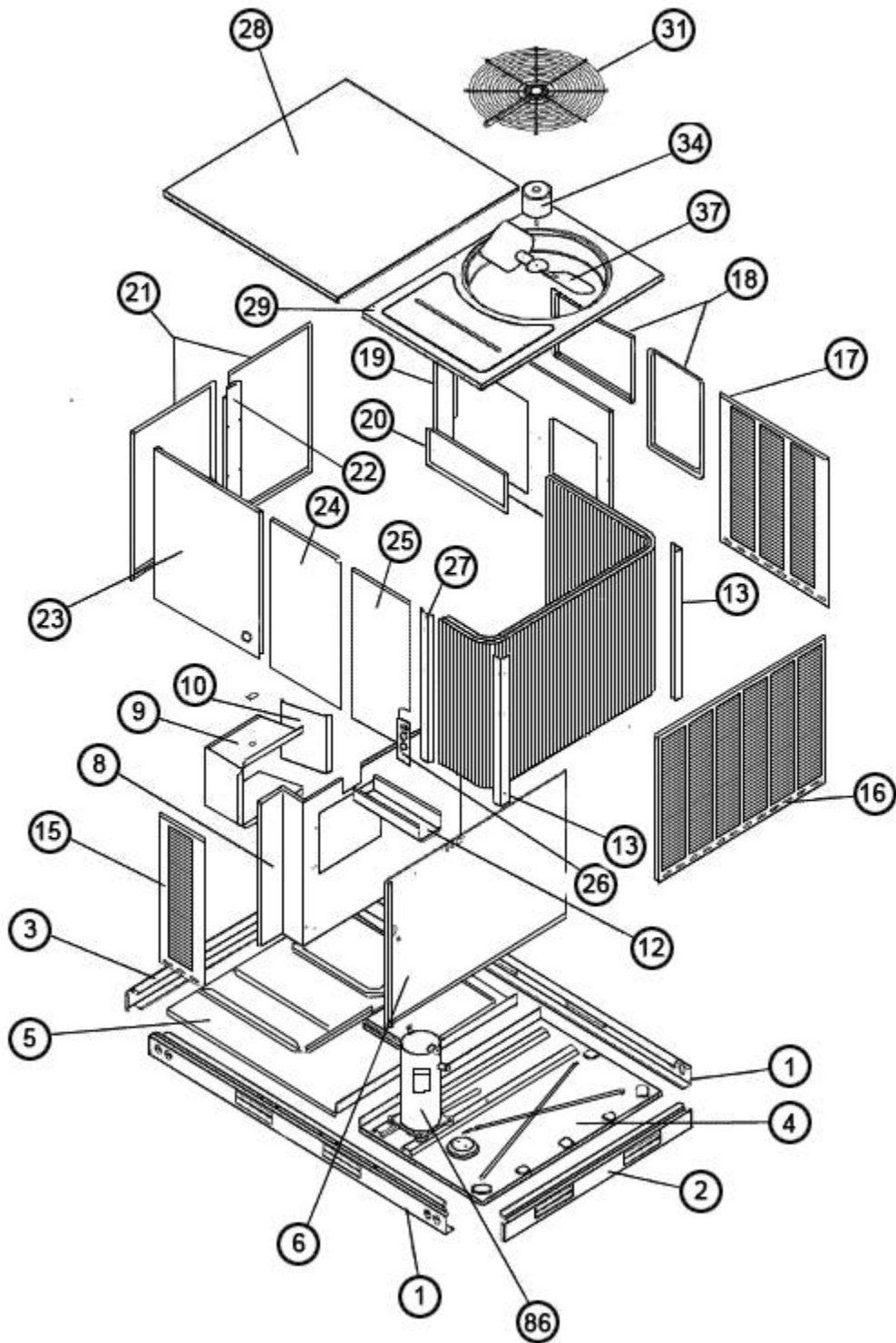
Exploded View
