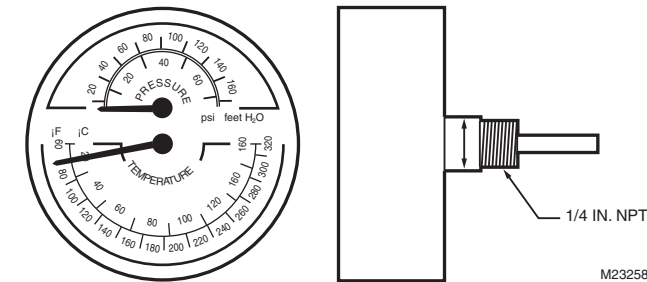
Dimensions Diagram
