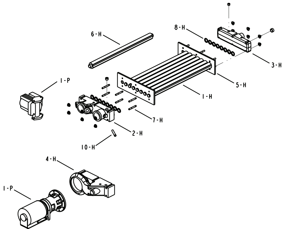
HEAT EXCHANGER DETAIL
