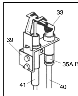
HONEYWELL IID PILOT
