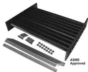
6234-101 006734F TUBE BUNDLE, ASME, CAST IRON HEADER
