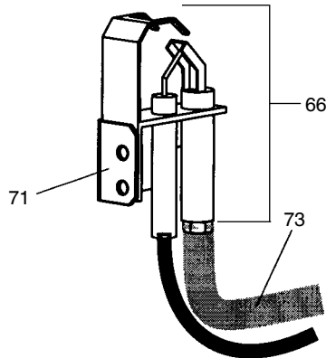
IID ATMOSPHERIC PILOT
