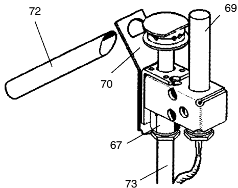
ATMOSPHERIC PILOT MILLOVOLT
