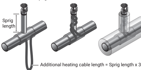
Figure 1.2 Installing XL-Trace Edge on the sprinklers
