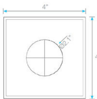
D Base - Top View
