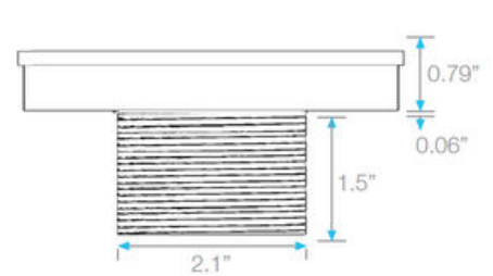
D Base - Side View
