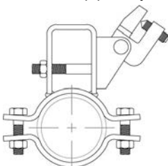
Lateral Brace
