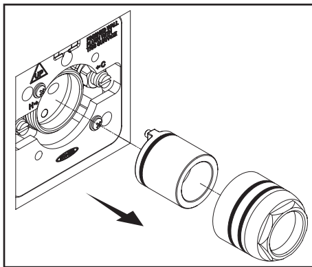
(2) Remove sleeve nut and test cap.
