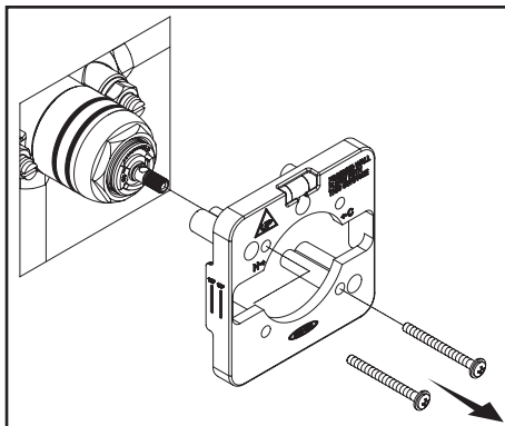
(5) Remove mud guard.
