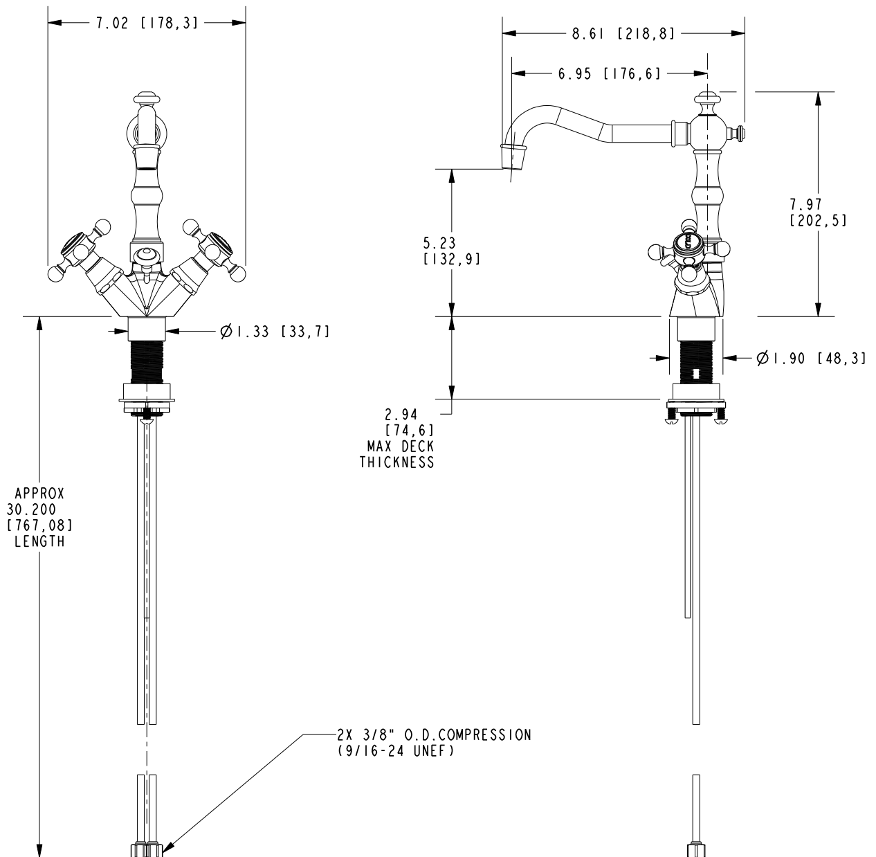
SINGLE HOLE LAVATORY FAUCET
